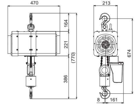
MLP-480K
