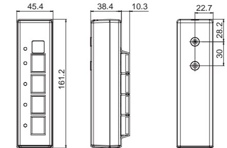
ML-RFC2
