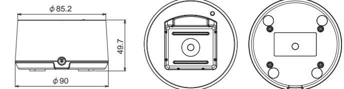
ML-WPT
